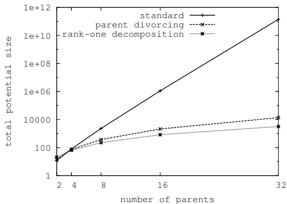
Figure 6: Comparison of the total size of junction tree.
