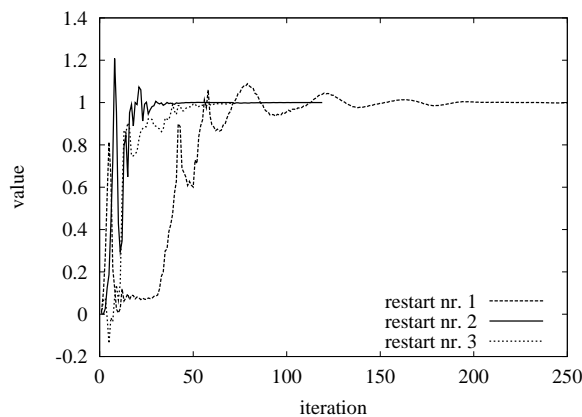
Figure 8: Development of one value of \psi' in case of decomposition of max.
