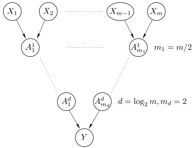
Figure 2: Bayesian network after parent divorcing.
