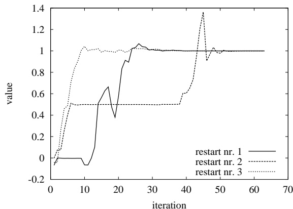
Figure 7: Development of one value of \psi' in case of decomposition of xor.
