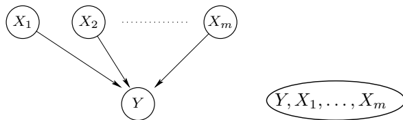
Figure 1: Bayesian network structure and its junction tree.
