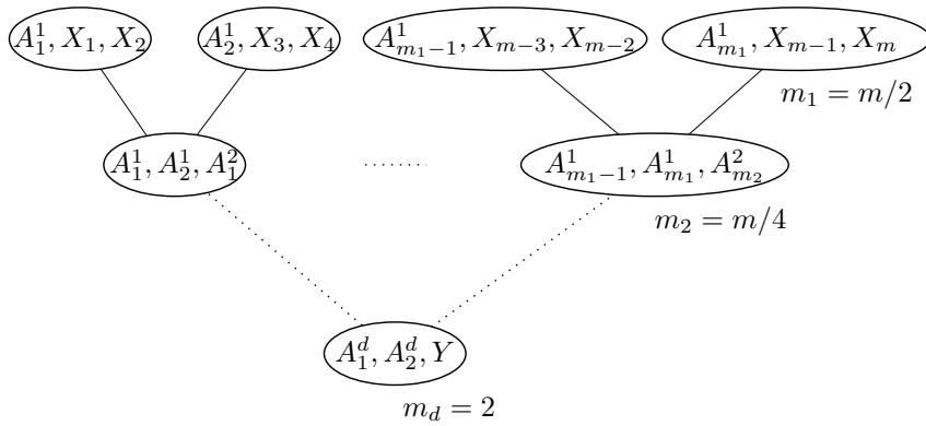
Figure 3: Junction tree for the parent divorcing method.
