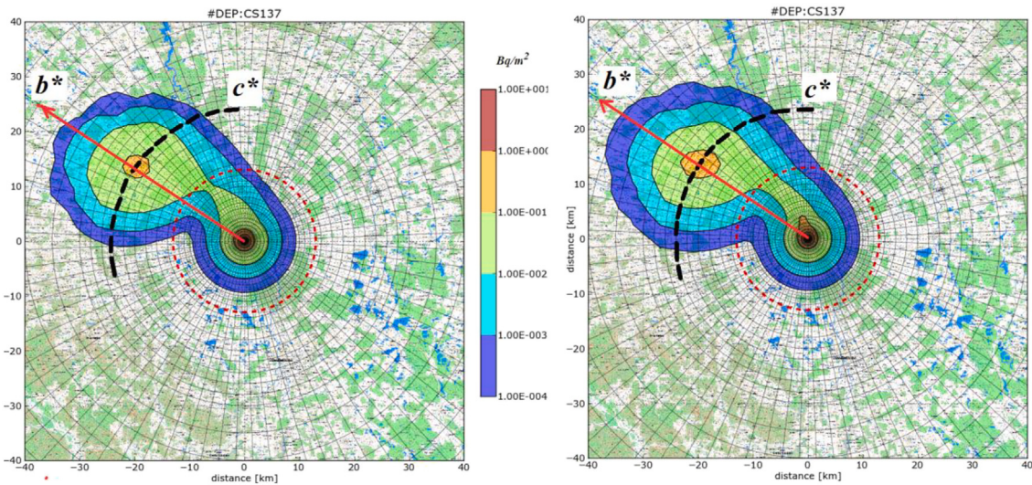
Fig. 9. The results for M = 100 for algorithms AB (Left) and BF (Right). The release scenario with the rain with intensity 1 \text{ mm}\cdot\text{h}^{-1} in the fourth phase (hour) of the convective transport. The peripheral circle c^* and the radial beam b^* of the polar computational grid are sketched.
