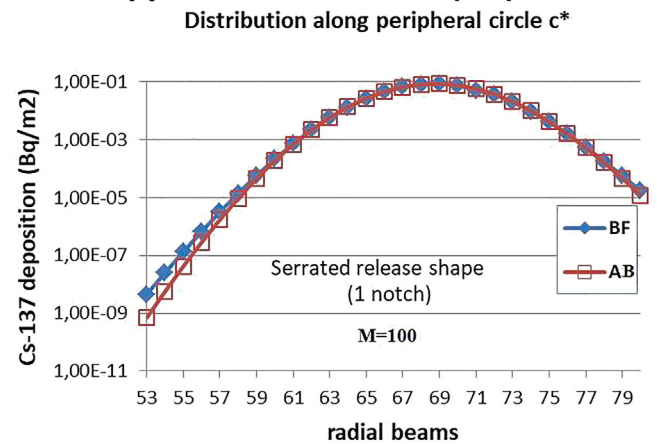
Fig. 12. The distribution of 137 Cs deposition on the ground in peripheral direction along the circle c* with diameter 25 km from the source as a function of the radial beams around beam b*=69 (sketched in Fig. 9). The values belong to the fourth rainy phase with the rain intensity 1 mm.h -1 .
