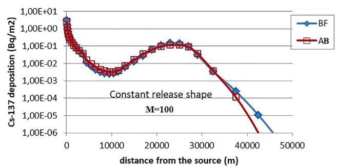
Fig. 11. The distribution of 137 Cs deposition on the ground in the radial direction along the beam b*=69 (shown in Fig. 9). The values concern the 4th rainy phase with the rain intensity 1 mm.h -1 .
