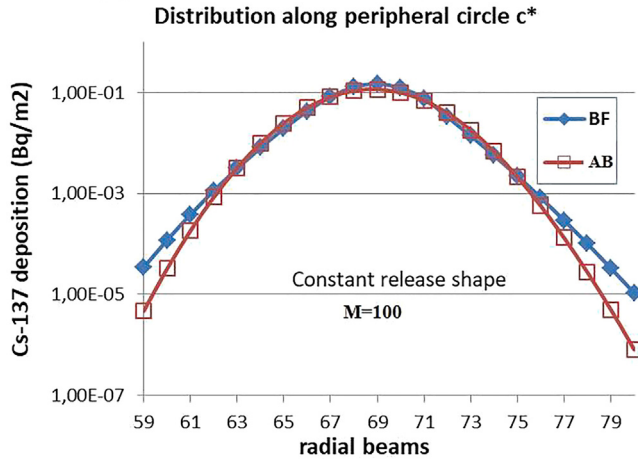
Fig. 10a. The distribution of 137 Cs deposition on the ground along the peripheral direction along the circle c* with diameter 25 km from the source as a function of the radial polar beams around beam b*=69 (sketched in Fig. 9). The values concern the fourth rainy phase with the rain intensity 1 mm.h -1 .
