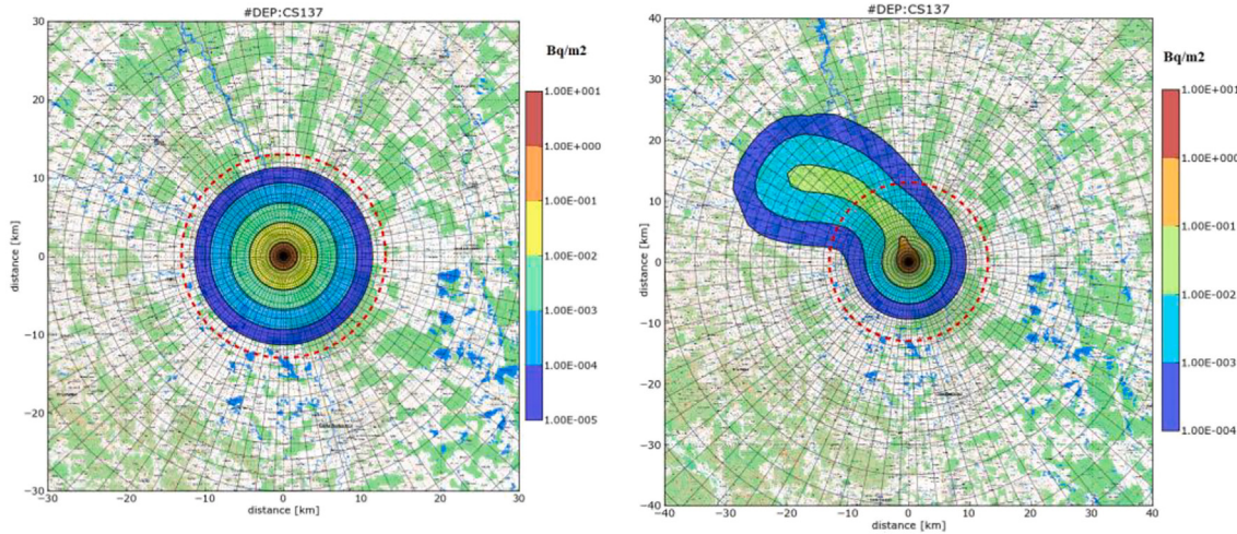
Fig. 6. Deposition of the radionuclide ^{137}\text{Cs} on terrain. No atmospheric precipitation, M = 100 , BF solution. Left panel: Detailed image of the deposition in the calm region in the emergency planning zone just after 5 h of the calm episode. Right: Deposition from a further propagation after the successive 4 h of the convective transport.
