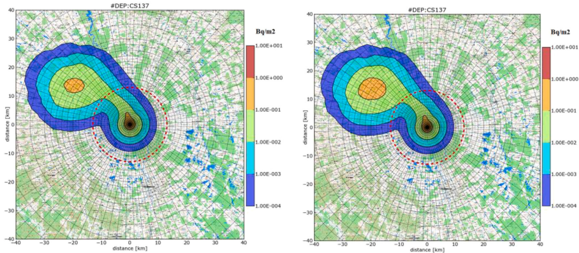
Fig. 7. “Hot spots” of deposited radionuclide ^{137}\text{Cs} on terrain. M = 100 , BF solution, the release source of a constant strength. The atmospheric precipitation in the fourth hour of the convective transport causes the serious increase of the deposited activity ^{137}\text{Cs} . Left: Results for the rain with the intensity 1.0 \text{ mm.h}^{-1} . Right: Rain with the higher intensity 2.0 \text{ mm.h}^{-1} .
