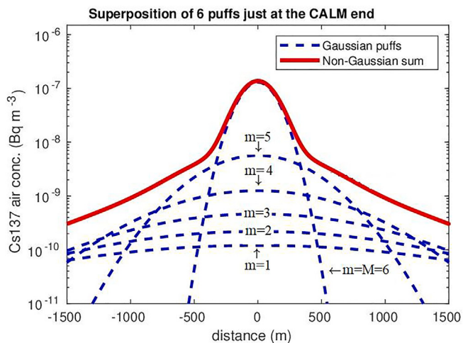
Fig. 3b. Similar results as on above Fig. 3a for analysis of minor calm scenario from (Pecha et al., 2020). Specific radioactivity of ^{137}\text{Cs} in air, all values related just to the end of the calm situation T_{END}^{CALM} . Composition of resulting non-Gaussian distribution (given by Eq. (3.1) - unbroken line) from the individual discrete Gaussian puffs m \in \{1, \dots, M\} ; M = 6 (dashed lines); Duration of the calm episode T^{CALM} = 2 h.
