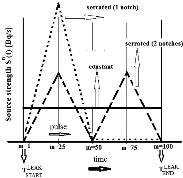
Fig. 5. The release source strength S^n(t) [ Bq \cdot s^{-1} ] for Case1 (constant shape), Case 2 (serrated, 2 notches) and Case 3 (serrated, 1 notch).
