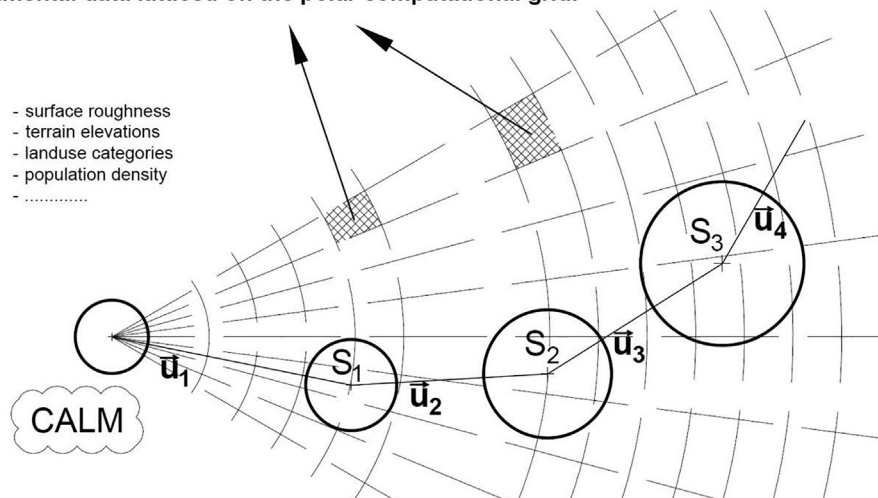
Fig. 4. Drift of the calm episode results in the ensuing convective flow. Each convective phase accounts for its specific environmental parameters. They are partially listed in the left upper corner.
