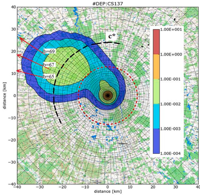
Fig. 8. “Hot spots” of deposited radionuclide ^{137}\text{Cs} on terrain. M = 100 , BF solution, serrated release source strength (Case 3 from Fig. 5: the serrated shape with one notch). Atmospheric precipitation with intensity 1.0 \text{ mm}\cdot\text{h}^{-1} in the fourth hour of the convective transport.
