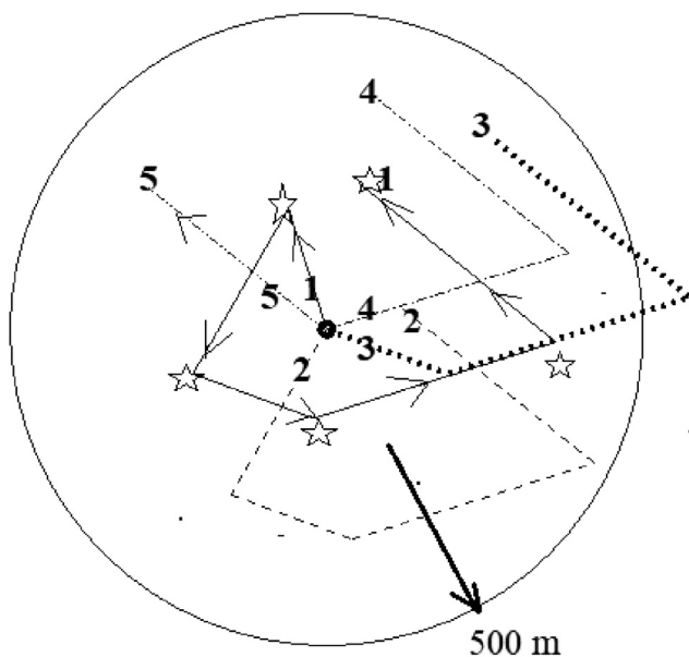
Fig. 1. Trajectories of five aerosol particles discharged at the source according the time stamps from Table 1. The depicted situation is just after the fifth hour 2,019,120,400 (Dec 04, 2019).
