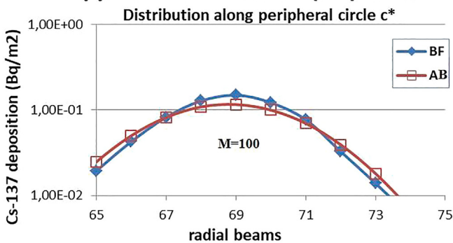
Fig. 10b. Zoom in the central region of Fig. 10a. Distribution of 137 Cs deposition on the ground along the peripheral direction along the circle c* with diameter 25 km from the source as a function of the radial polar beams around beam b*=69 (sketched in Fig. 9).
