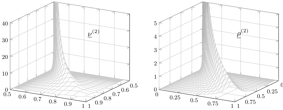
FIG. 2. The nontrivial solutions \underline{\nu}^{(2)} and \underline{\rho}^{(2)} of the bivariate RDE for frozen percolation on the oriented binary tree and the MBBT, respectively. Plotted are the densities of the restrictions of the measures to [\frac{1}{2}, 1]^2 and [0, 1]^2 , respectively.
