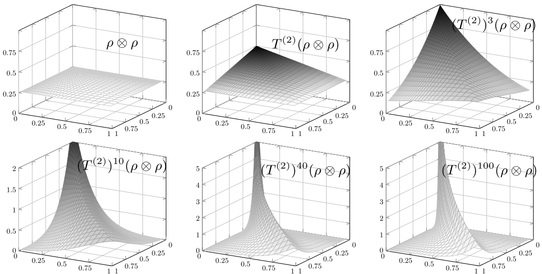
FIG. 3. Iterating the bivariate map T^{(2)} on the product measure \rho \otimes \rho produces a series of measures that by (1.11) converge to the nontrivial fixed point \underline{\rho}^{(2)} . Plotted is the density of the restriction of (T^{(2)})^n(\rho \otimes \rho) to the unit square for n = 0, 1, 3, 10, 40, and 100 . The last plot is already very close to the theoretical limit.
