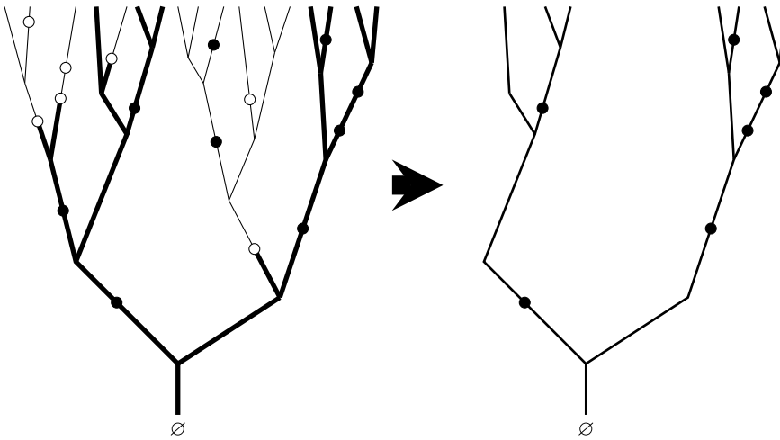
FIG. 1. Scaling of the marked binary branching tree. On the left: At time t , points in \Pi_t are still closed and marked with white circles, while points in \Pi_0 \setminus \Pi_t have already opened and are marked with black circles. On the right: Removing the loose ends from the open cluster at the root yields a stretched version of the original marked binary branching tree.
